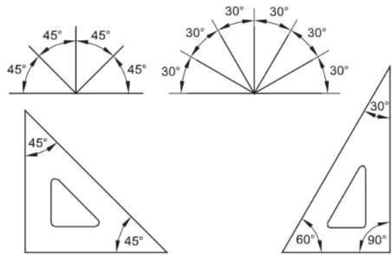
(a) 45° SET SQUARE
