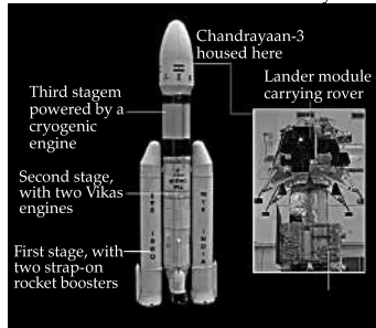
The LVM3 launch Rocket and Chandrayaan-3
