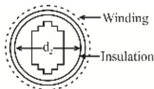
Stepped core transformer
